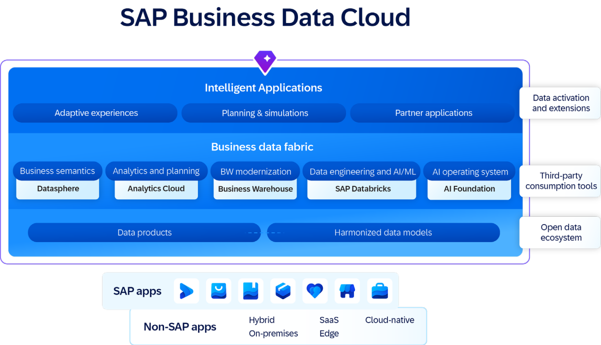
Figure 1: Architecture of SAP Business Data Cloud
